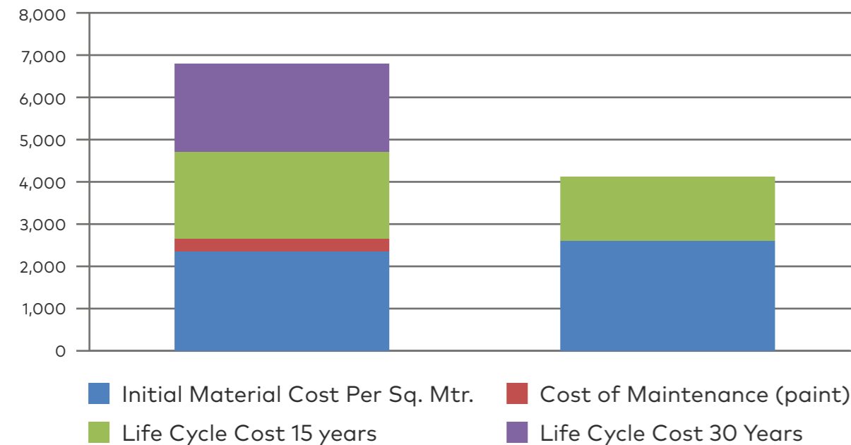
LCC of SS 409M HRAP Chequered vs Mild Steel HF Chequered Over 30 Years Life
